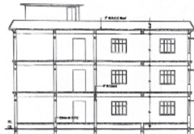
SECTION ON O-P BLOCK - B
