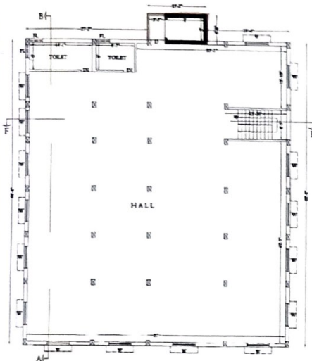
EXISTING FIRST & SECOND FLOOR PLAN WITH EXTENSION BLOCK - A
