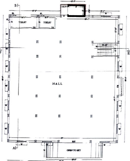
EXISTING GROUND FLOOR PLAN WITH EXTENSION BLOCK - A
