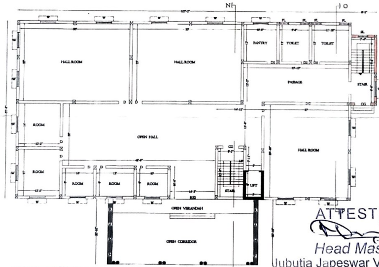
EXISTING GROUND FLOOR PLAN WITH EXTENSION BLOCK - B
