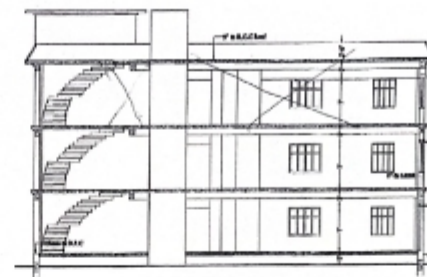
SECTION ON G-D BLOCK - C
