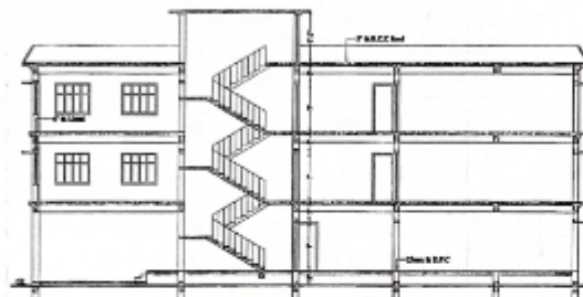
SECTION ON M-N BLOCK - B
