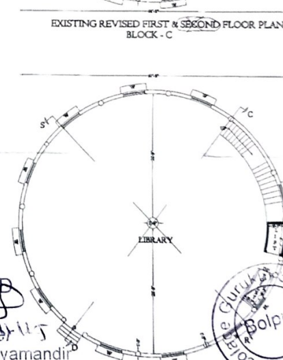
EXISTING REVISED GROUND FLOOR PLAN BLOCK - C
